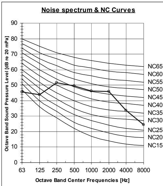
YGF024 Cooling
