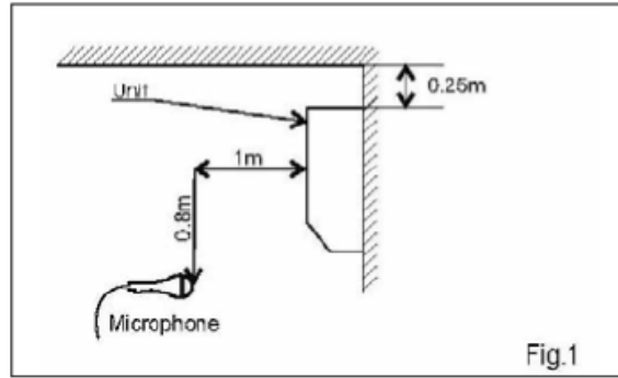
Figure 1. Wall Mounted
