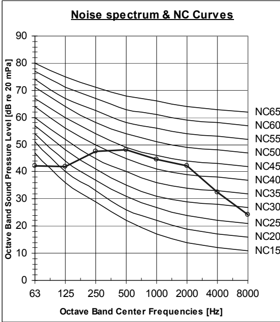
YGF009 Cooling
