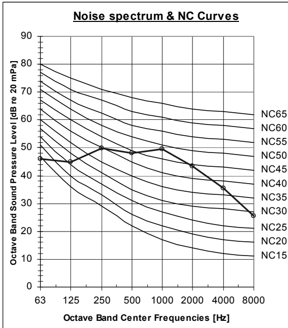
YGF018 Cooling
