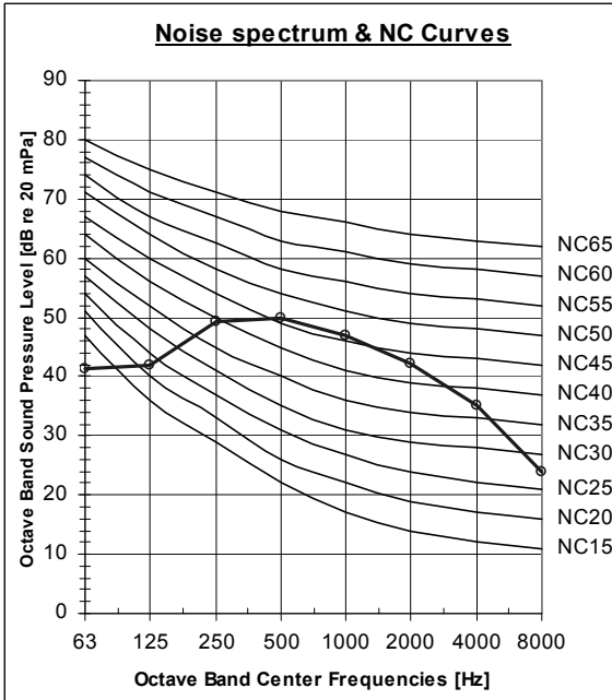
YGF012 Cooling
